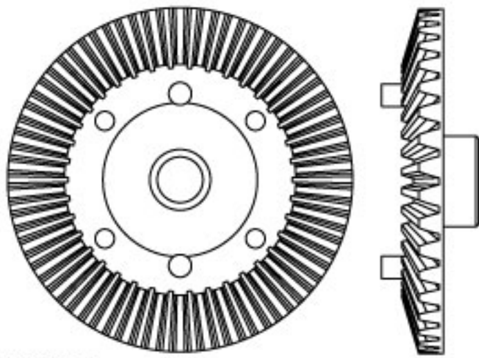
AX30392 38T Bevel Gear x1
