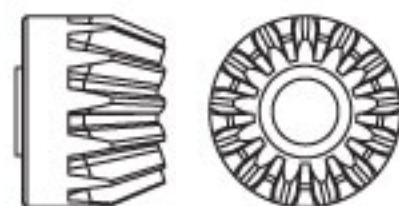
AX30392 13T Bevel Gear x2
